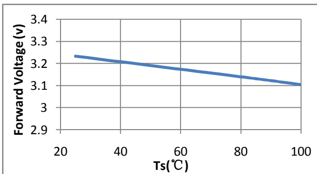
Fig.5-Forward Voltage Vs. Temperature 电压与温度特性曲线
