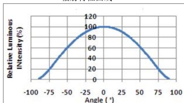
Fig.6-Radiation diagram
