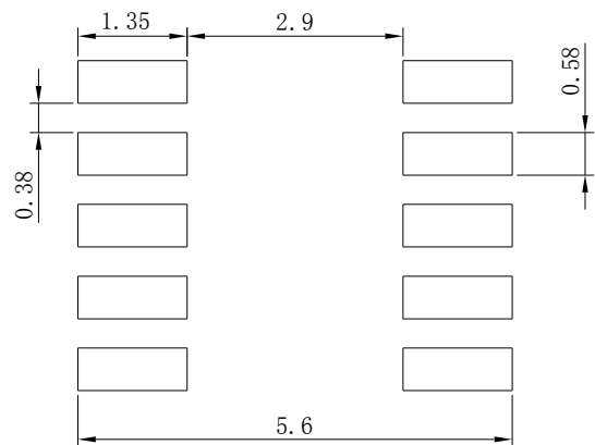
Soldering Patterns
